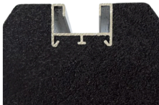
NEW T BAR DESIGN TO CREATE A STRONGER BOND
